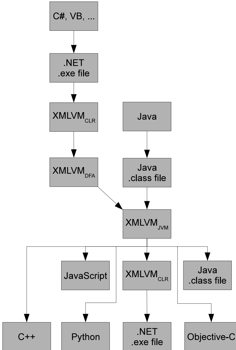
Figure 1.1: XMLVM Toolchain.
